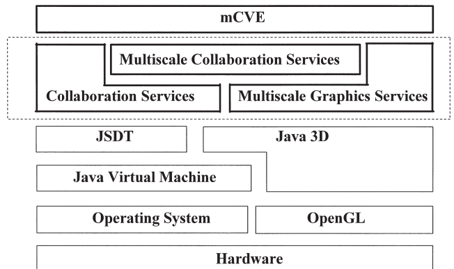
Figure 9. System layer of the mCVE prototype.
